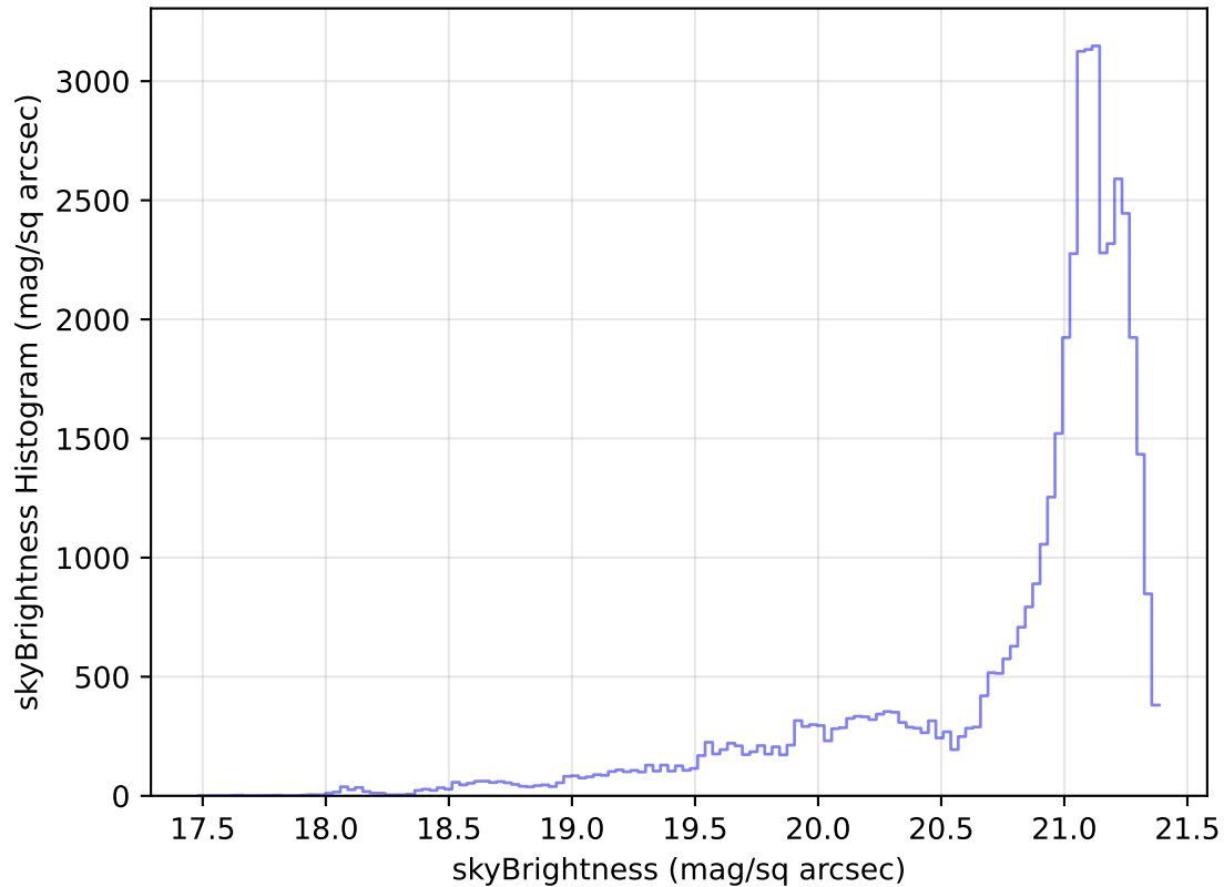
internal_u_expt45_nscale0.9v3.4_10yrs Yr 1 r band: skyBrightness Histogram
