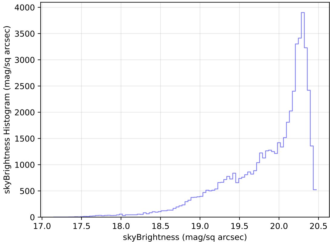
internal_u_expt45_nscale0.9v3.4_10yrs Yr 1 i band: skyBrightness Histogram
