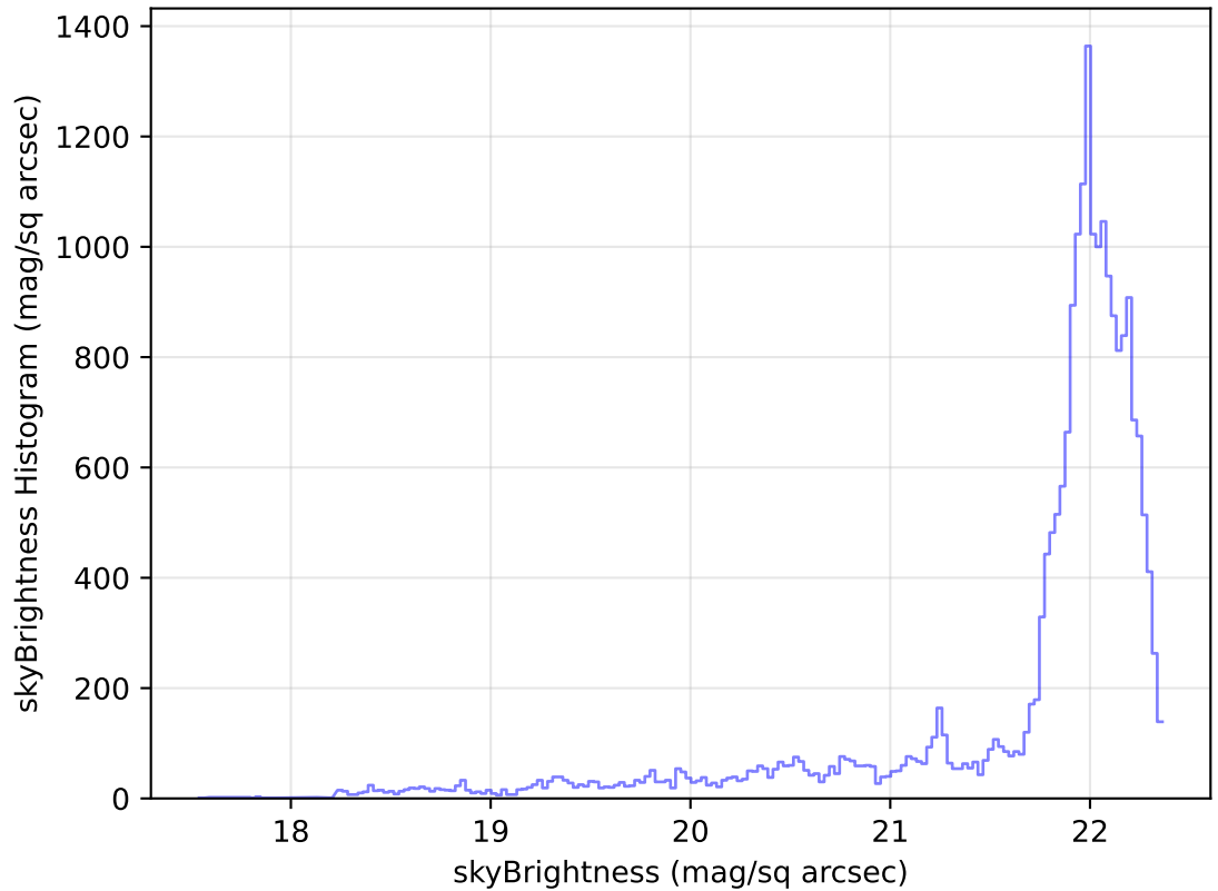
internal_u_expt45_nscale0.9v3.4_10yrs Yr 1 g band: skyBrightness Histogram
