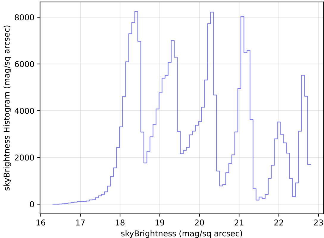
internal_u_expt45_nscale0.9v3.4_10yrs Yr 1 all bands: skyBrightness Histogram
