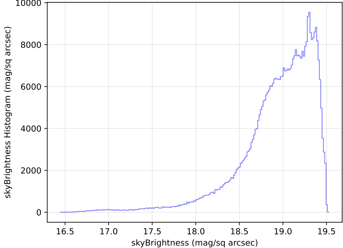
internal_u_expt45_nscale0.9v3.4_10yrs WFD z band: skyBrightness Histogram
