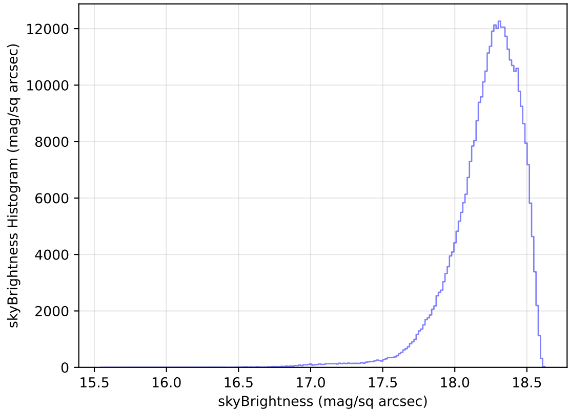
internal_u_expt45_nscale0.9v3.4_10yrs WFD y band: skyBrightness Histogram
