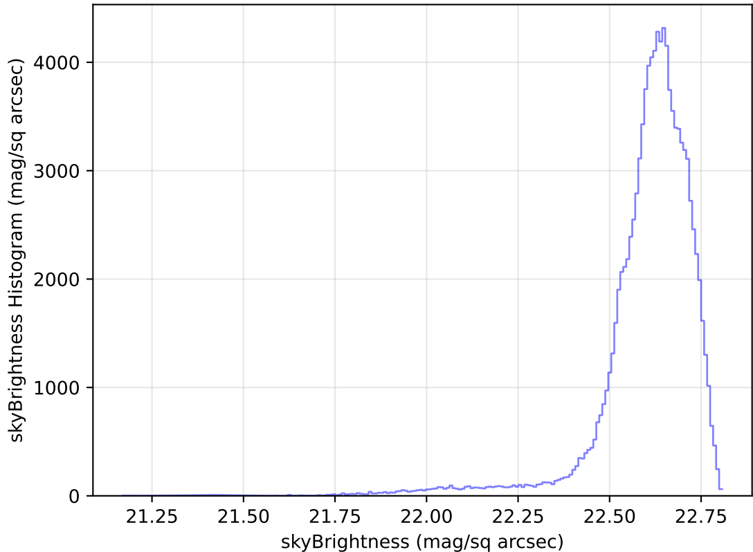
internal_u_expt45_nscale0.9v3.4_10yrs WFD u band: skyBrightness Histogram
