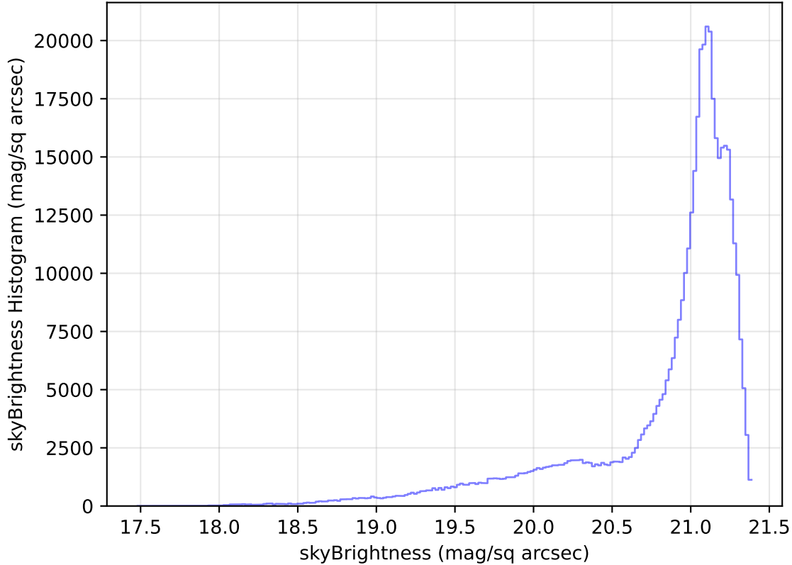
internal_u_expt45_nscale0.9v3.4_10yrs WFD r band: skyBrightness Histogram
