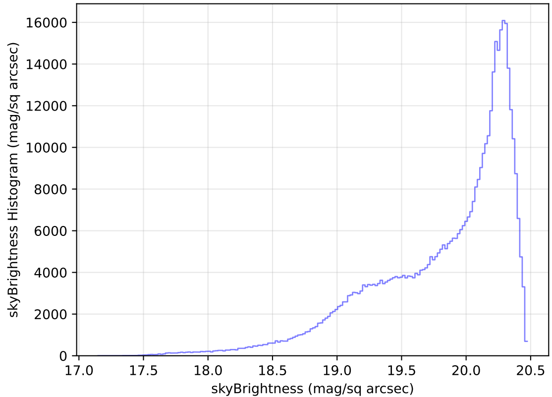
internal_u_expt45_nscale0.9v3.4_10yrs WFD i band: skyBrightness Histogram
