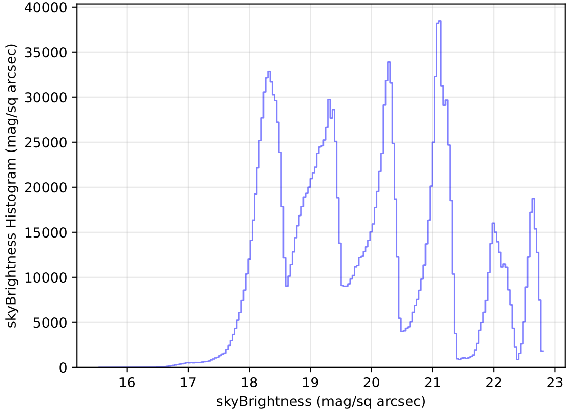
internal_u_expt45_nscale0.9v3.4_10yrs WFD all bands: skyBrightness Histogram
