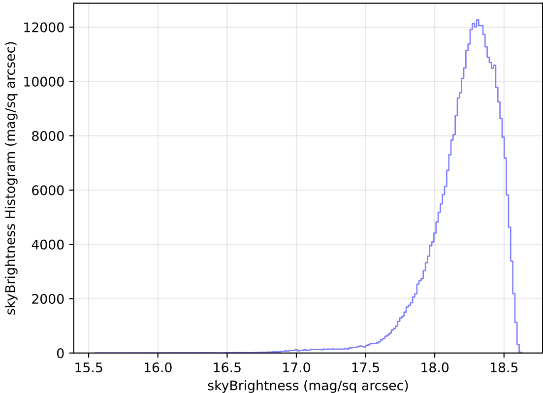
internal_u_expt45_nscale0.9v3.4_10yrs All sky y band: skyBrightness Histogram
