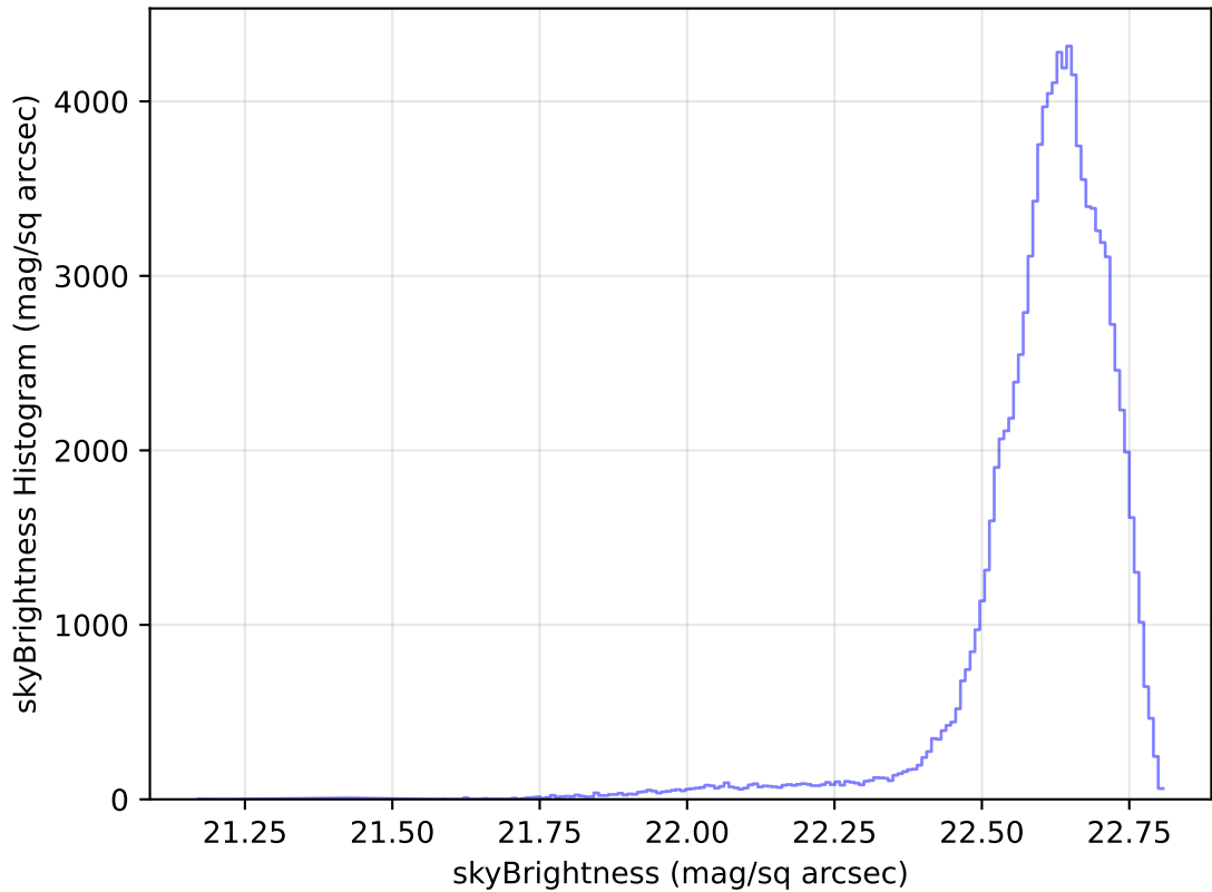
internal_u_expt45_nscale0.9v3.4_10yrs All sky u band: skyBrightness Histogram
