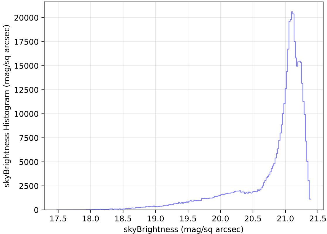
internal_u_expt45_nscale0.9v3.4_10yrs All sky r band: skyBrightness Histogram
