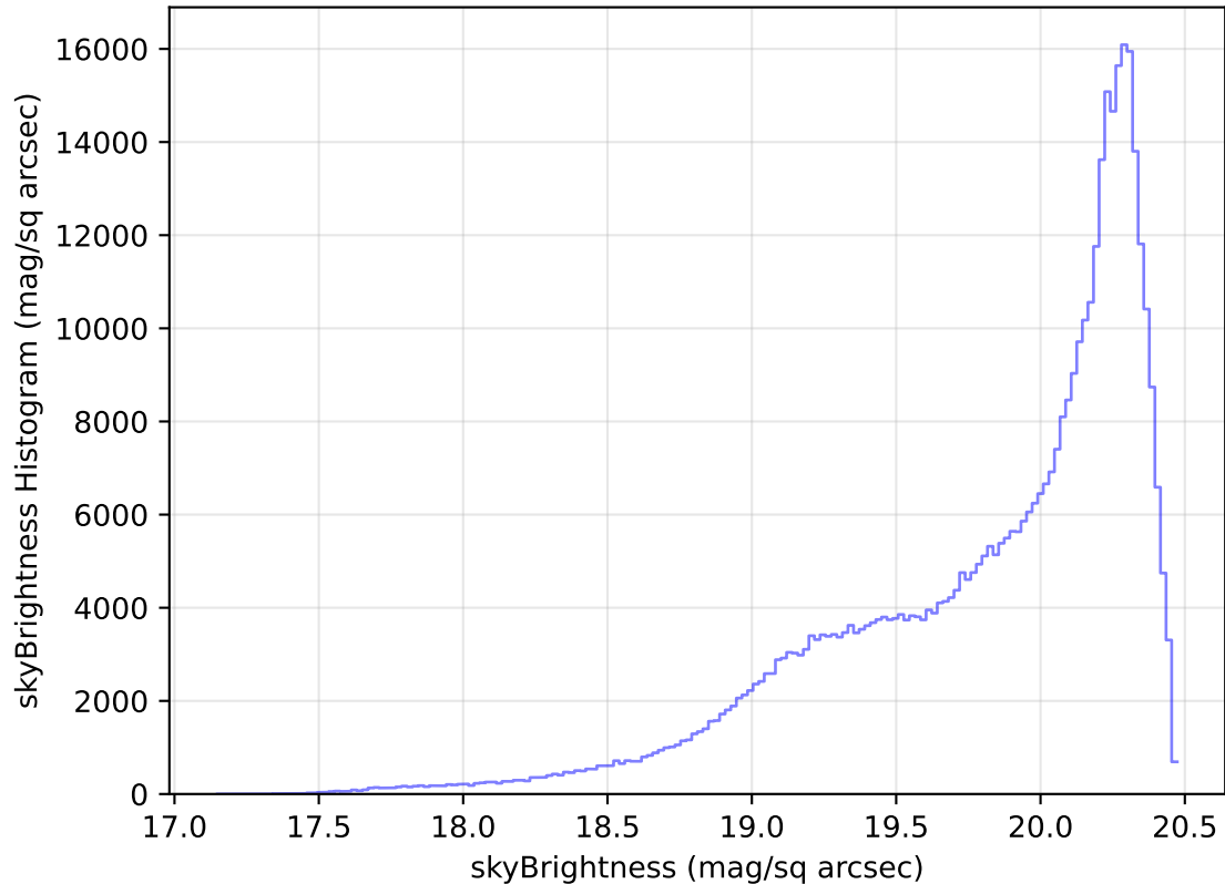
internal_u_expt45_nscale0.9v3.4_10yrs All sky i band: skyBrightness Histogram
