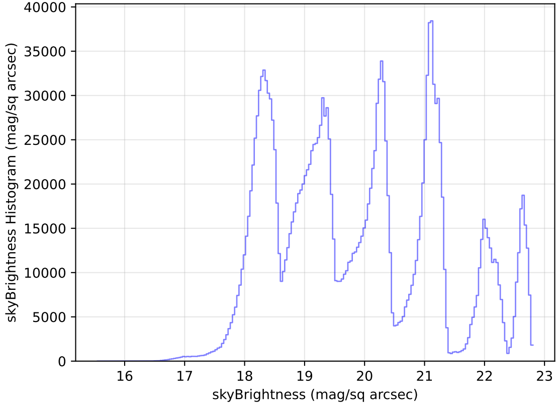
internal_u_expt45_nscale0.9v3.4_10yrs All sky all bands: skyBrightness Histogram
