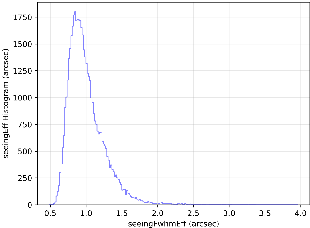
internal_u_expt45_nscale0.9v3.4_10yrs Yr 1 y band: seeingEff Histogram
