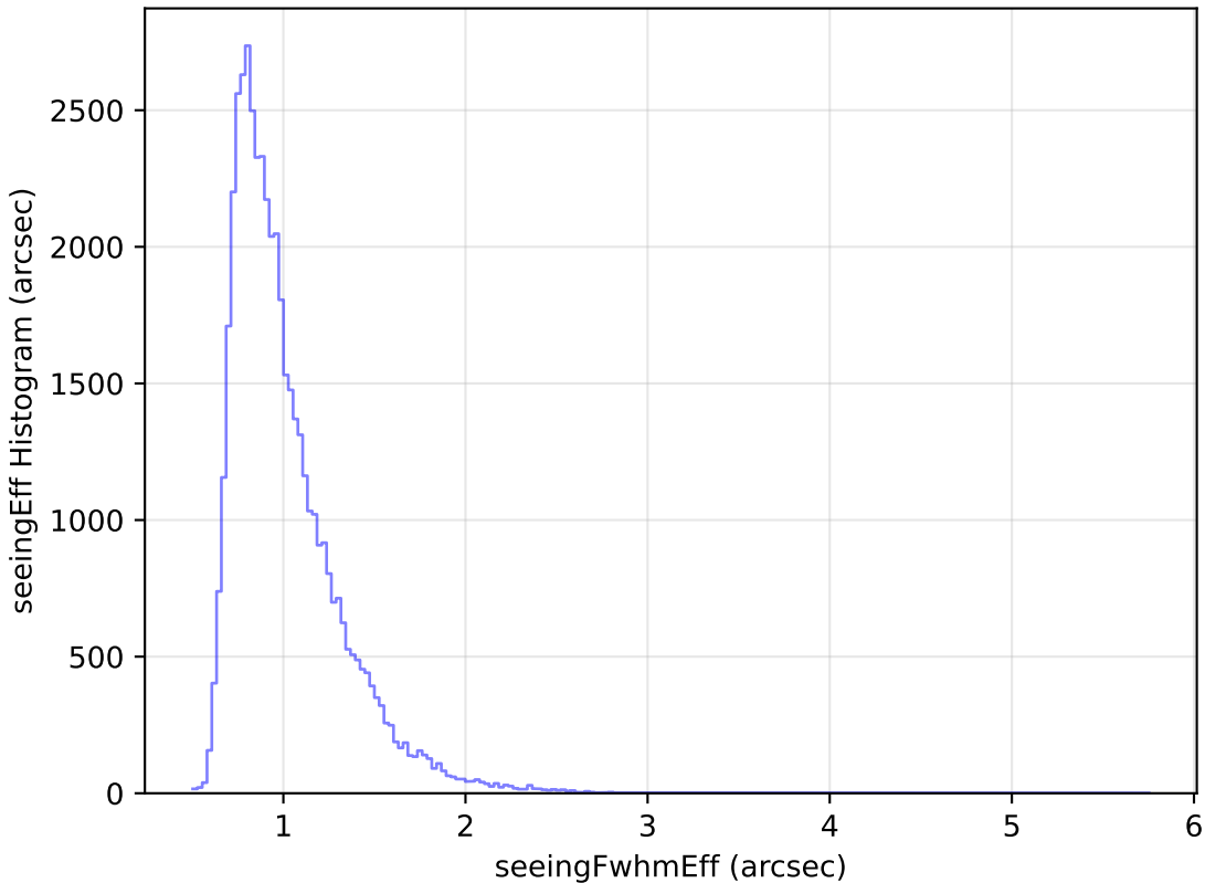
internal_u_expt45_nscale0.9v3.4_10yrs Yr 1 r band: seeingEff Histogram
