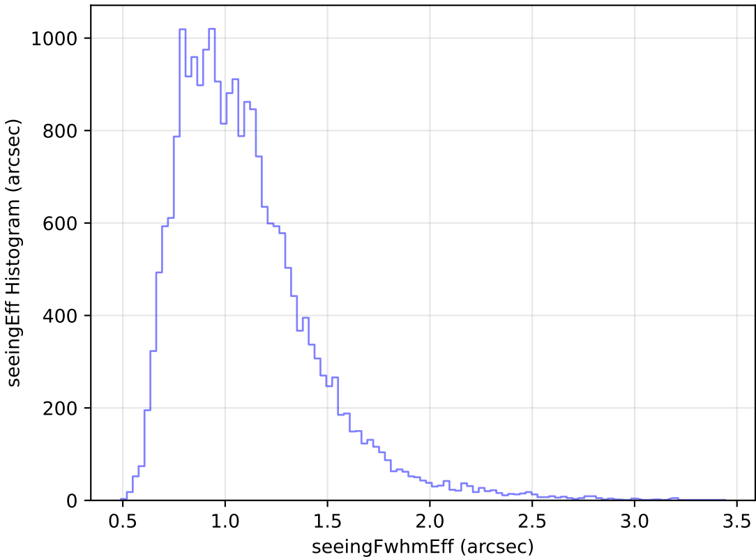
internal_u_expt45_nscale0.9v3.4_10yrs Yr 1 g band: seeingEff Histogram
