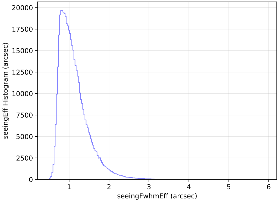
internal_u_expt45_nscale0.9v3.4_10yrs WFD r band: seeingEff Histogram
