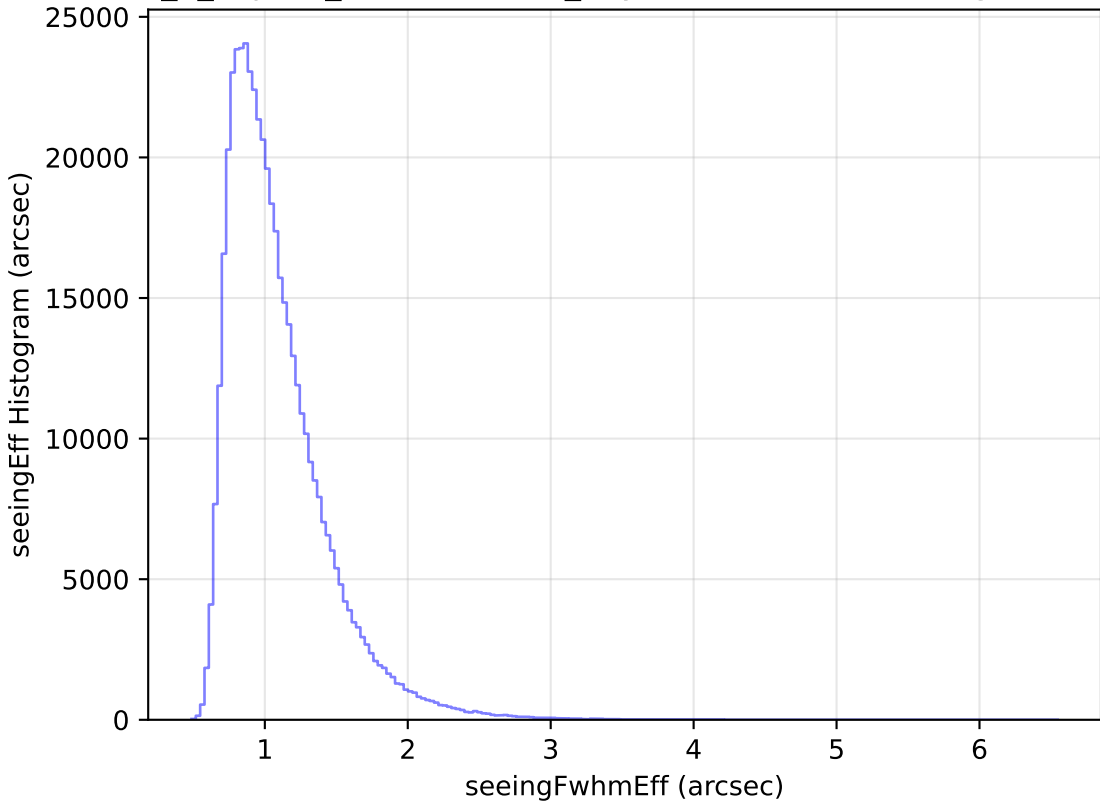
internal_u_expt45_nscale0.9v3.4_10yrs WFD i band: seeingEff Histogram
