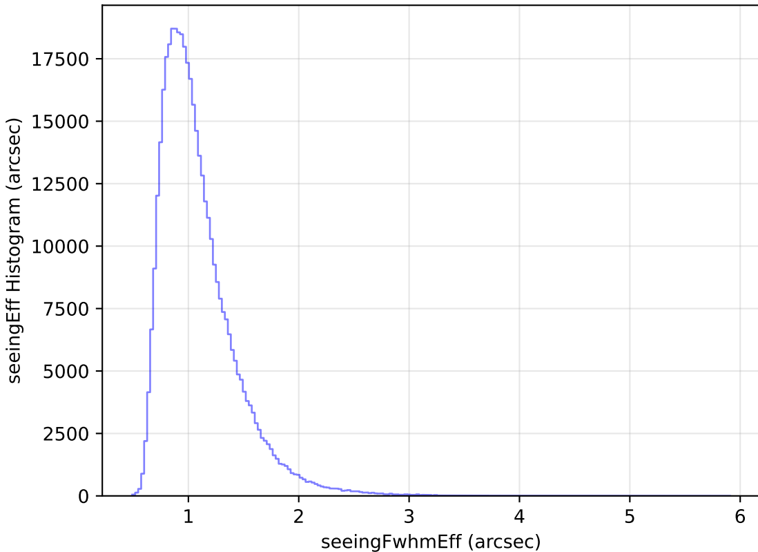
internal_u_expt45_nscale0.9v3.4_10yrs All sky z band: seeingEff Histogram
