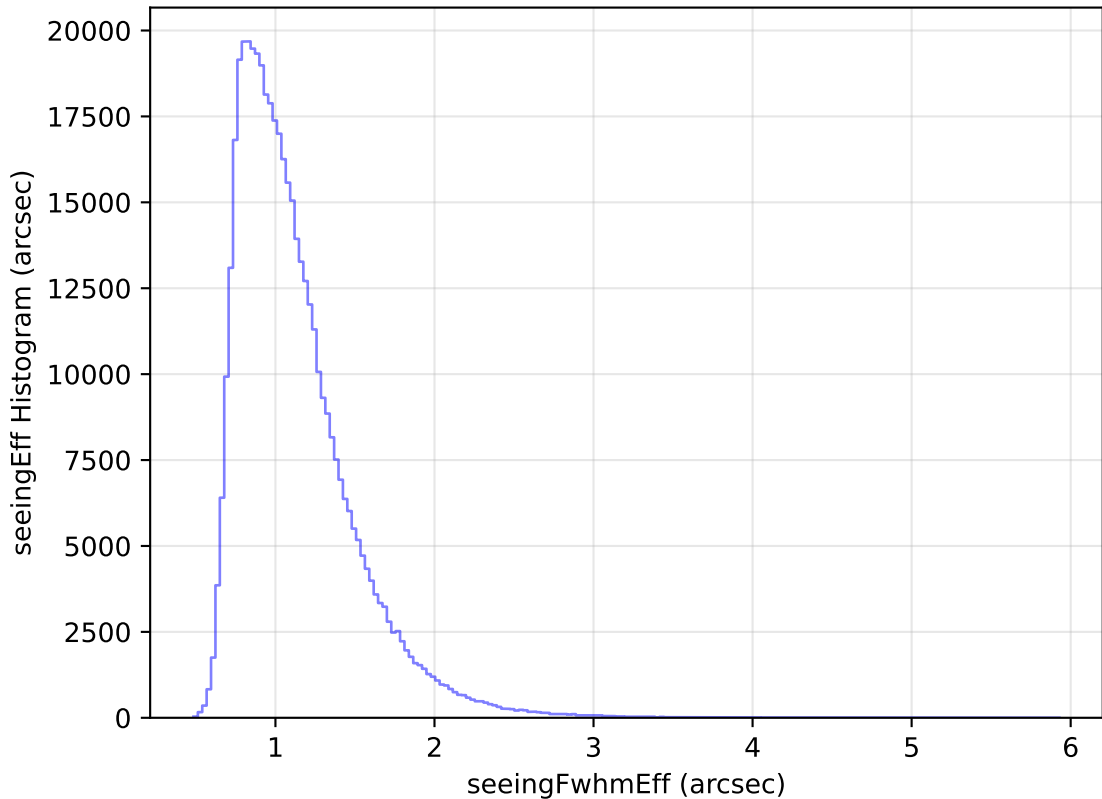
internal_u_expt45_nscale0.9v3.4_10yrs All sky r band: seeingEff Histogram
