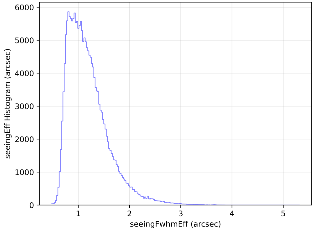
internal_u_expt45_nscale0.9v3.4_10yrs All sky g band: seeingEff Histogram
