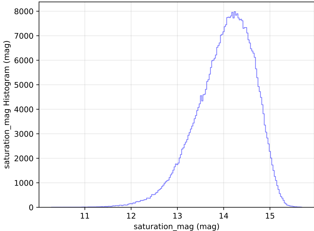
internal_u_expt45_nscale0.9v3.4_10yrs WFD z band: saturation_mag Histogram
