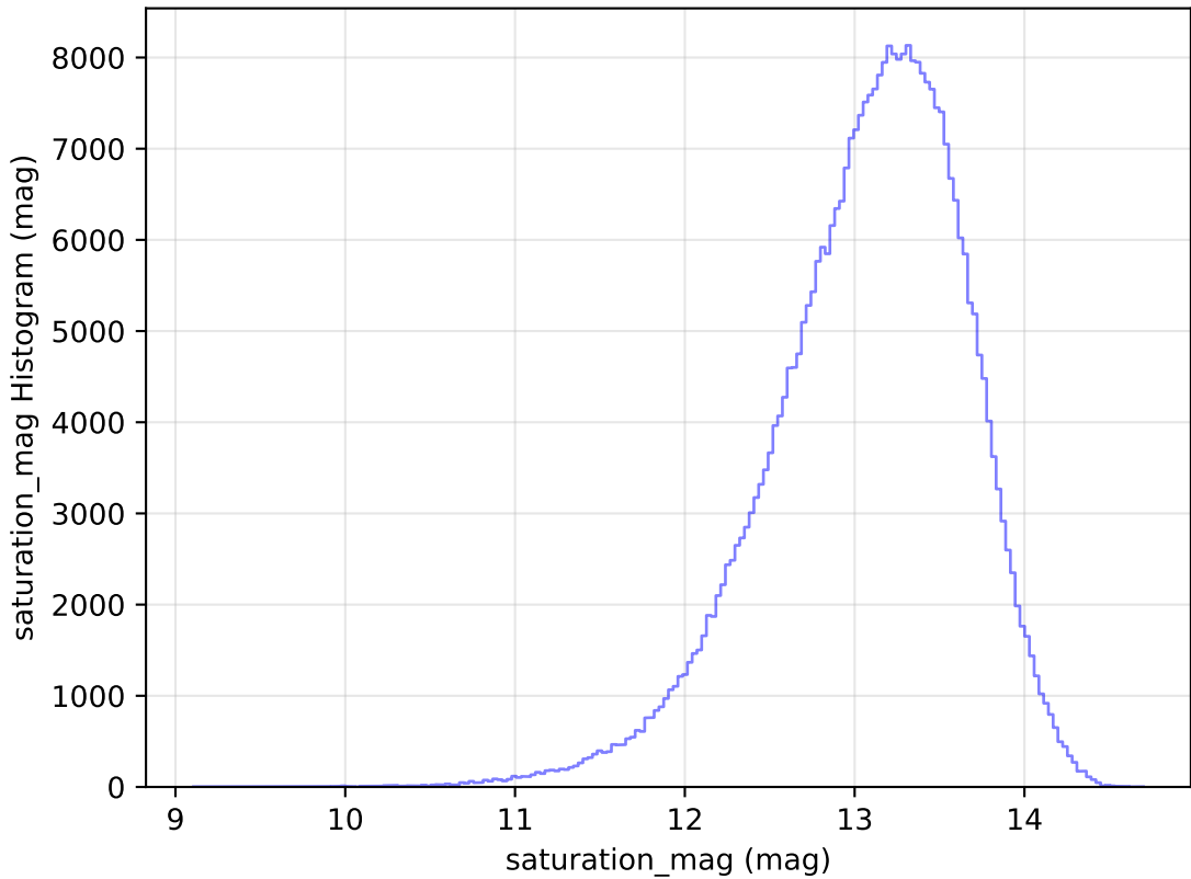
internal_u_expt45_nscale0.9v3.4_10yrs WFD y band: saturation_mag Histogram
