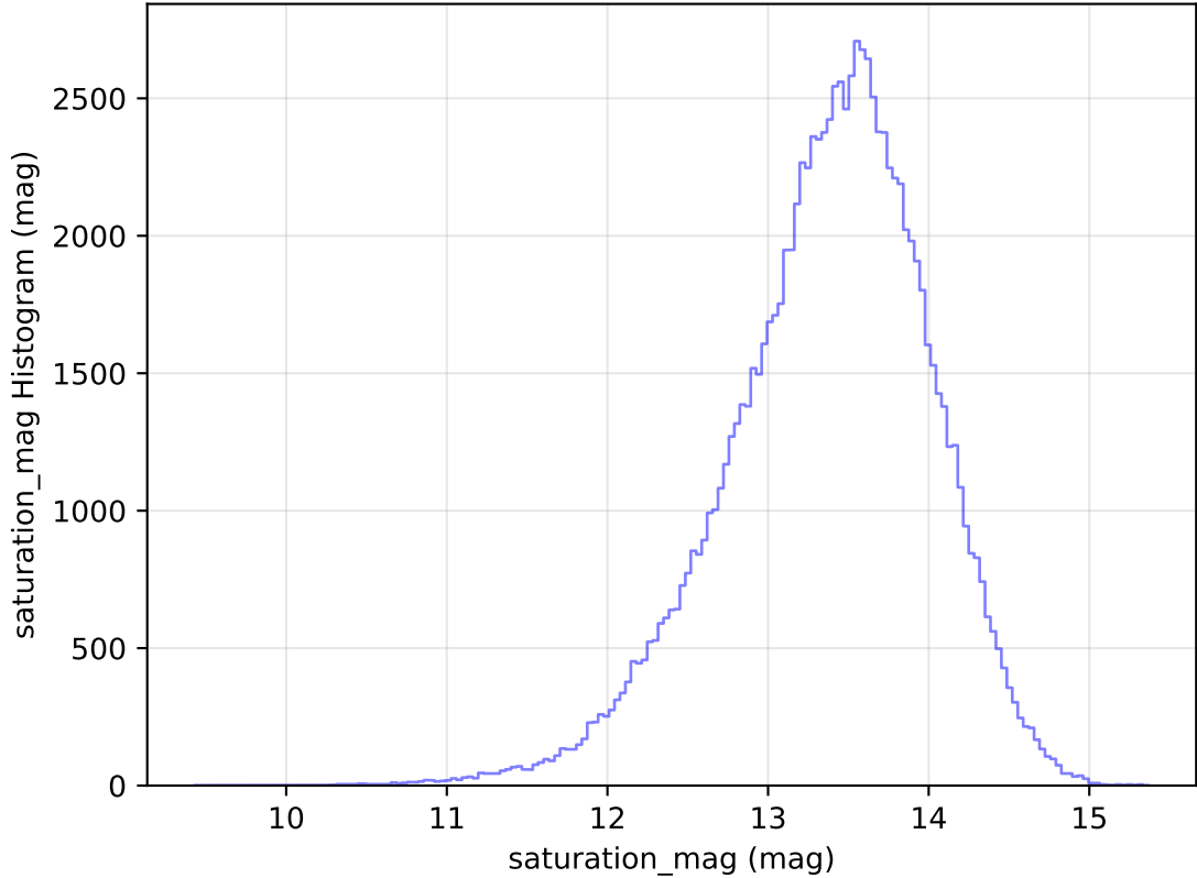
internal_u_expt45_nscale0.9v3.4_10yrs WFD u band: saturation_mag Histogram
