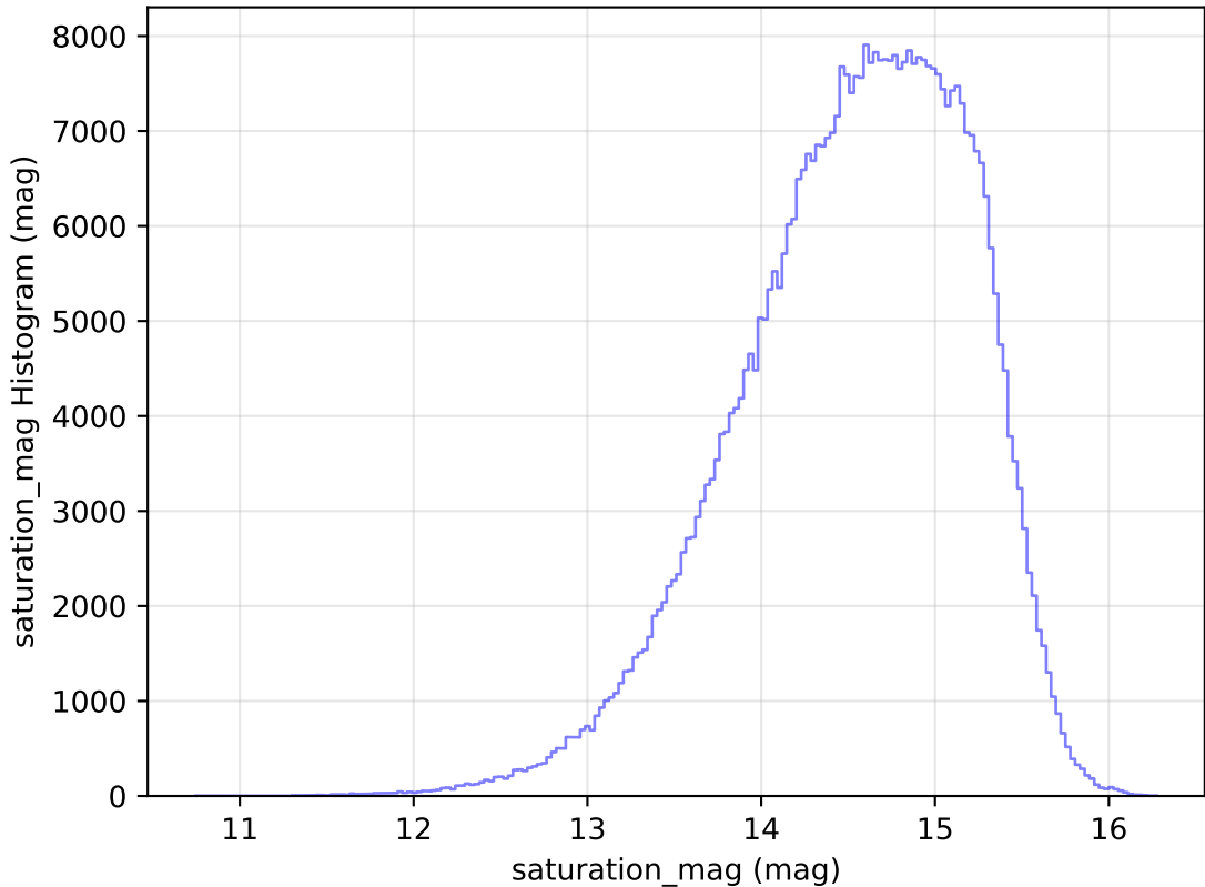
internal_u_expt45_nscale0.9v3.4_10yrs WFD r band: saturation_mag Histogram
