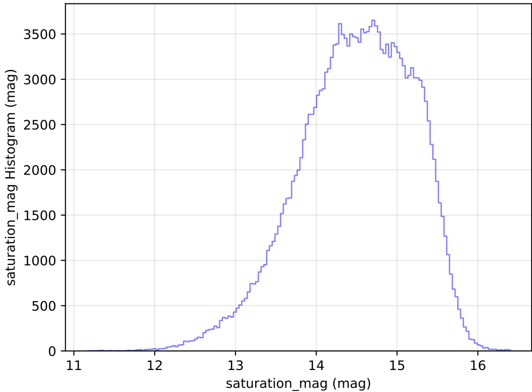
internal_u_expt45_nscale0.9v3.4_10yrs WFD g band: saturation_mag Histogram
