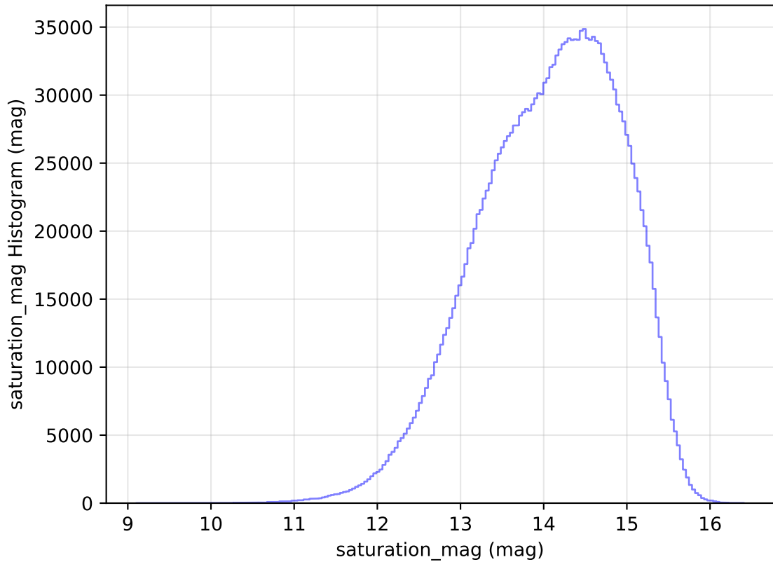
internal_u_expt45_nscale0.9v3.4_10yrs WFD all bands: saturation_mag Histogram
