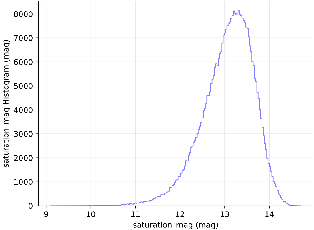
internal_u_expt45_nscale0.9v3.4_10yrs All sky y band: saturation_mag Histogram
