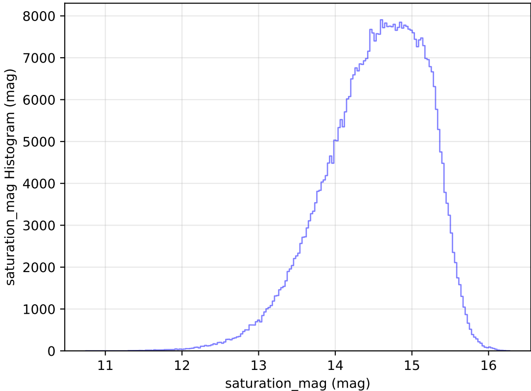
internal_u_expt45_nscale0.9v3.4_10yrs All sky r band: saturation_mag Histogram
