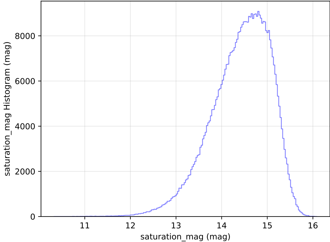
internal_u_expt45_nscale0.9v3.4_10yrs All sky i band: saturation_mag Histogram
