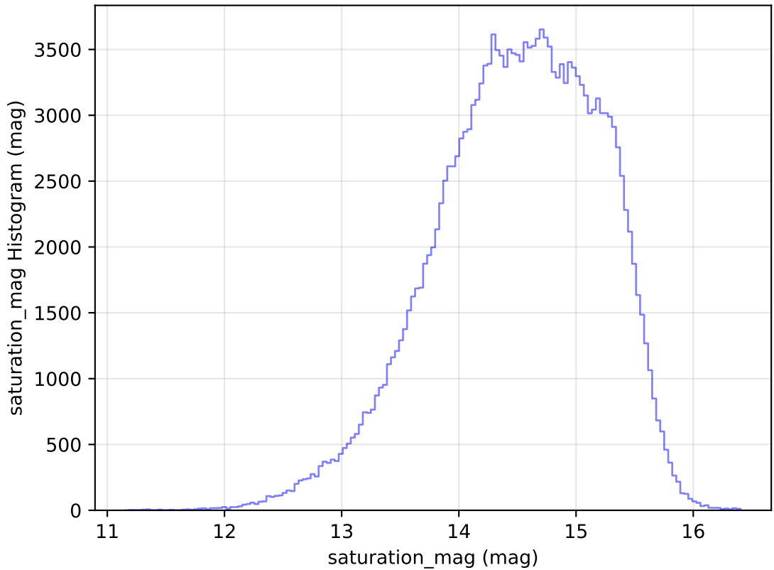
internal_u_expt45_nscale0.9v3.4_10yrs All sky g band: saturation_mag Histogram
