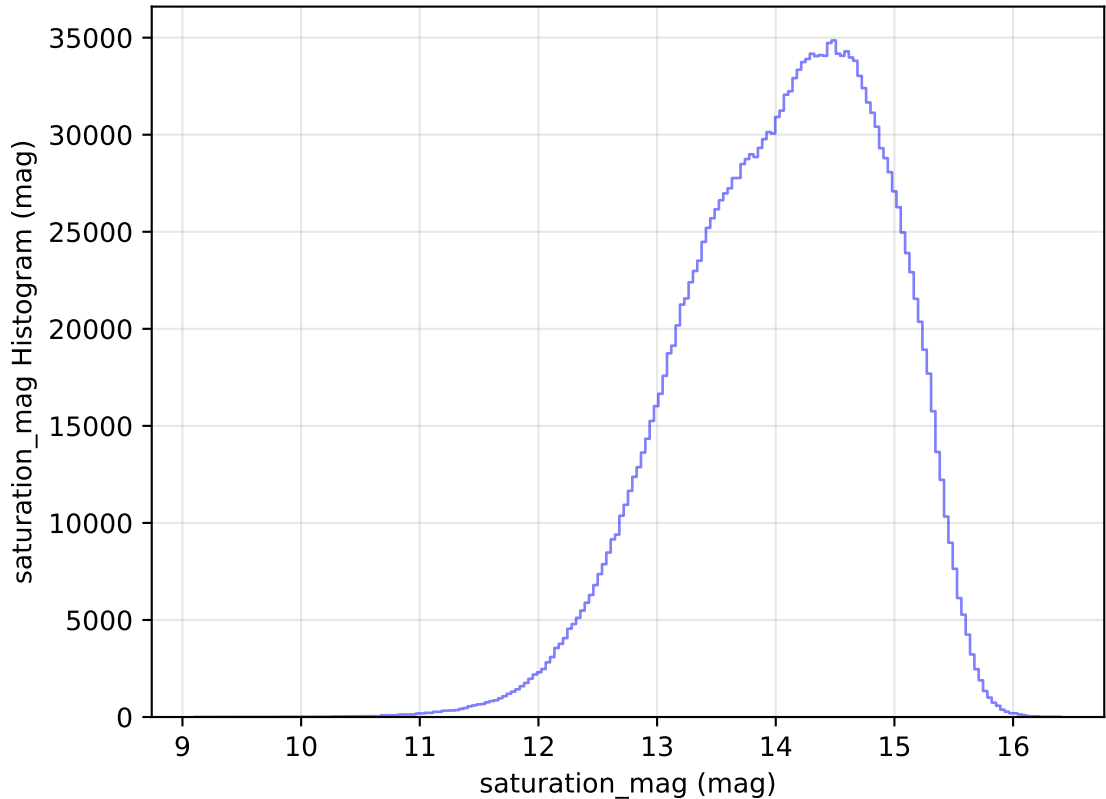
internal_u_expt45_nscale0.9v3.4_10yrs All sky all bands: saturation_mag Histogram
