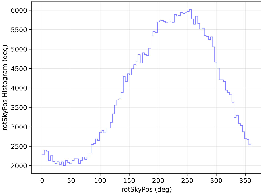
internal_u_expt45_nscale0.9v3.4_10yrs WFD y band: rotSkyPos Histogram
