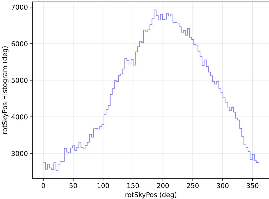
internal_u_expt45_nscale0.9v3.4_10yrs WFD r band: rotSkyPos Histogram
