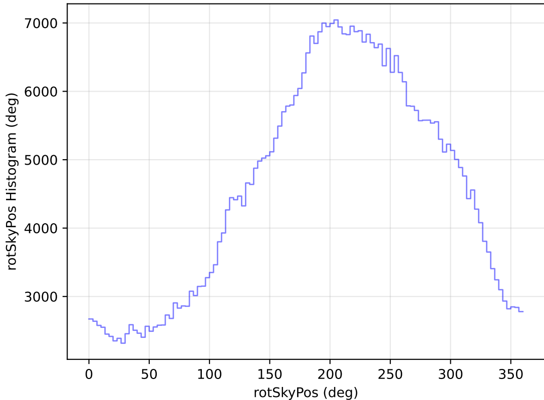
internal_u_expt45_nscale0.9v3.4_10yrs WFD i band: rotSkyPos Histogram
