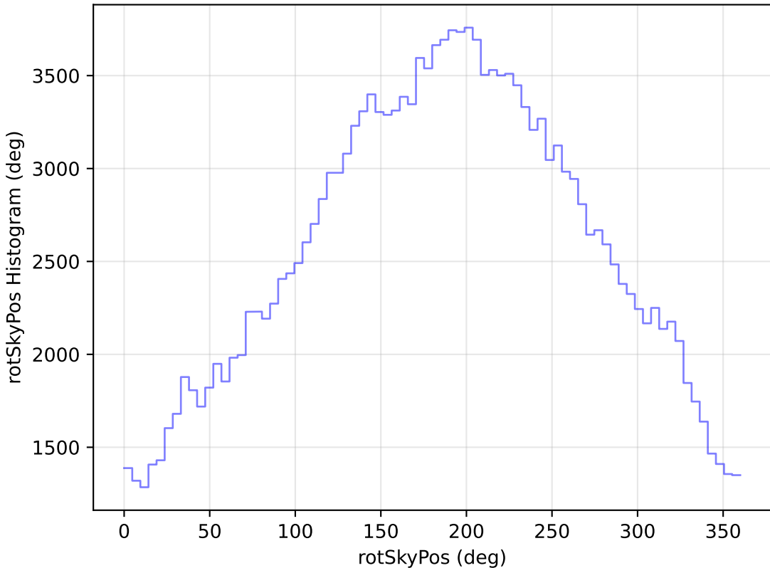
internal_u_expt45_nscale0.9v3.4_10yrs WFD g band: rotSkyPos Histogram
