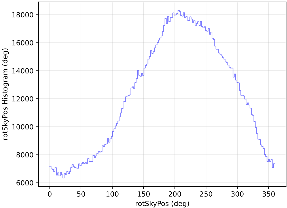
internal_u_expt45_nscale0.9v3.4_10yrs WFD all bands: rotSkyPos Histogram
