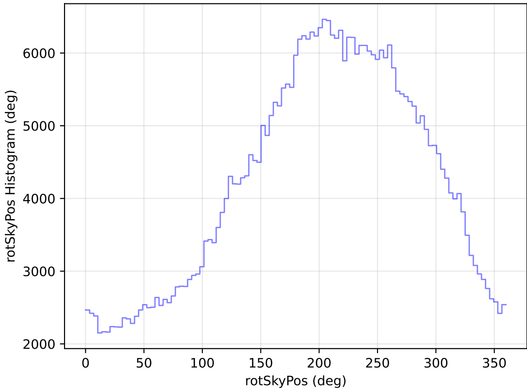
internal_u_expt45_nscale0.9v3.4_10yrs All sky z band: rotSkyPos Histogram
