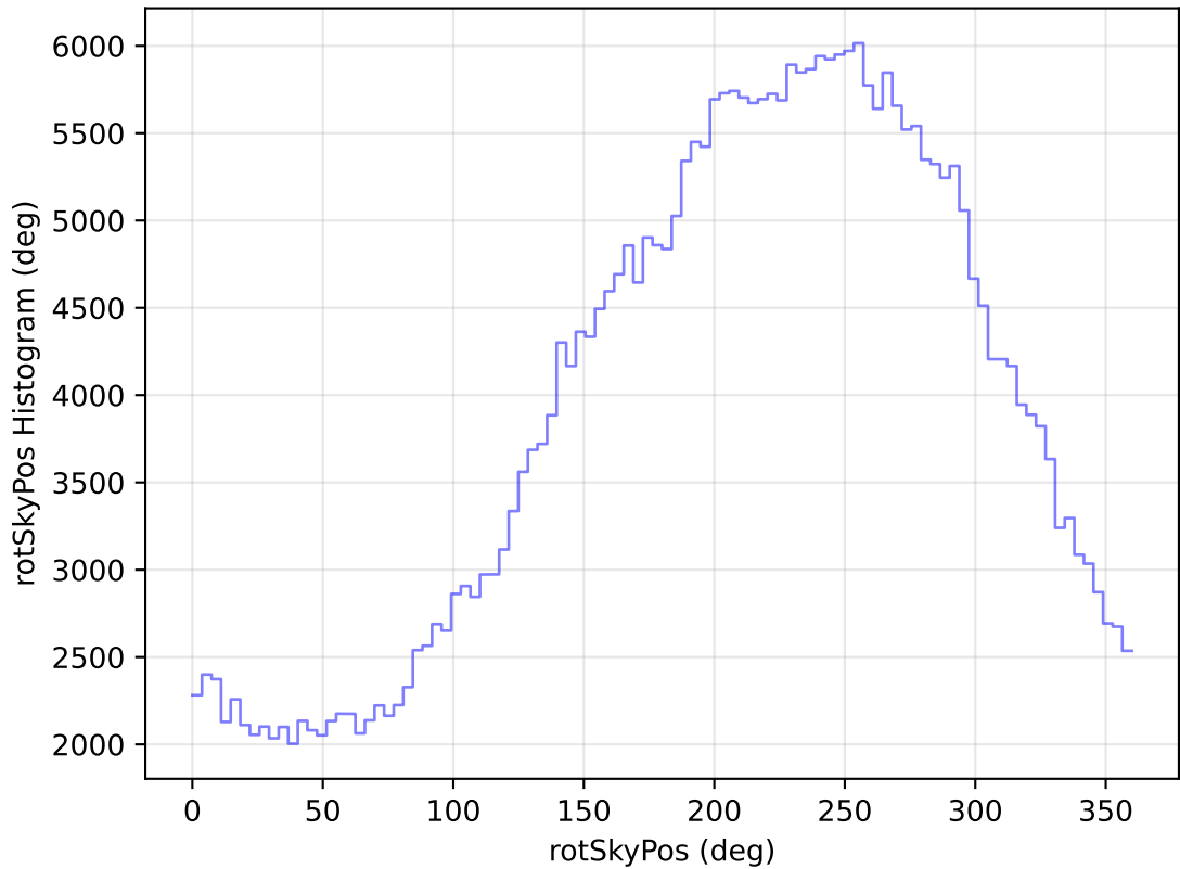
internal_u_expt45_nscale0.9v3.4_10yrs All sky y band: rotSkyPos Histogram
