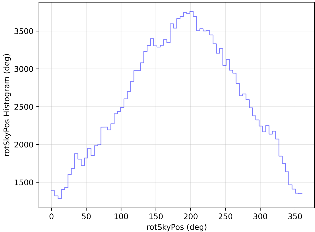
internal_u_expt45_nscale0.9v3.4_10yrs All sky g band: rotSkyPos Histogram
