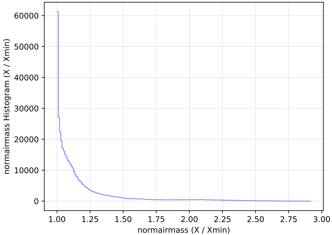
internal_u_expt45_nscale0.9v3.4_10yrs WFD z band: normairmass Histogram
