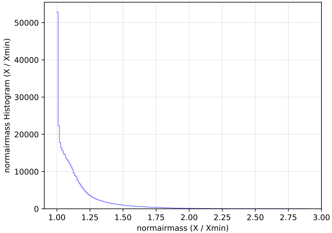
internal_u_expt45_nscale0.9v3.4_10yrs WFD y band: normairmass Histogram
