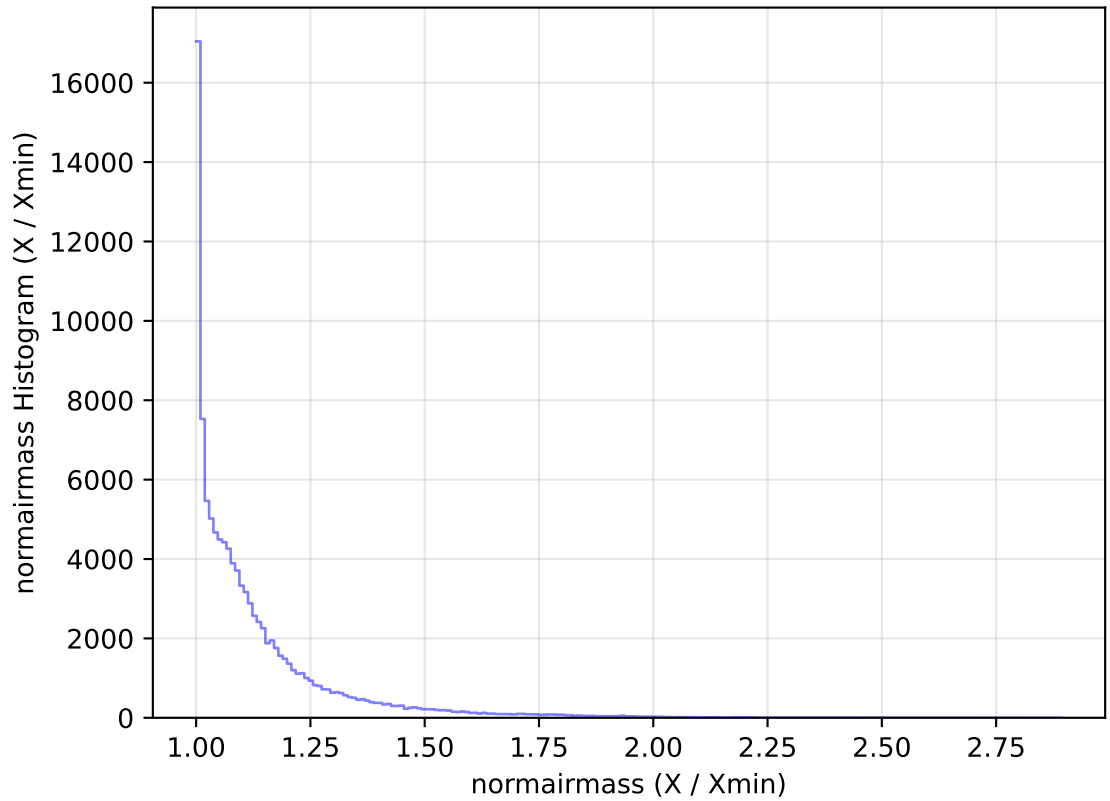
internal_u_expt45_nscale0.9v3.4_10yrs WFD u band: normairmass Histogram
