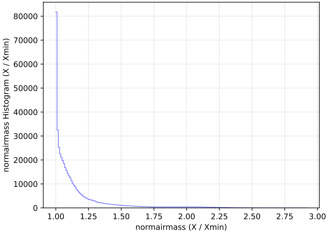
internal_u_expt45_nscale0.9v3.4_10yrs WFD r band: normairmass Histogram
