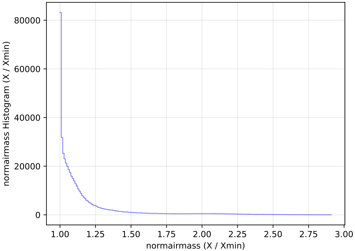
internal_u_expt45_nscale0.9v3.4_10yrs WFD i band: normairmass Histogram
