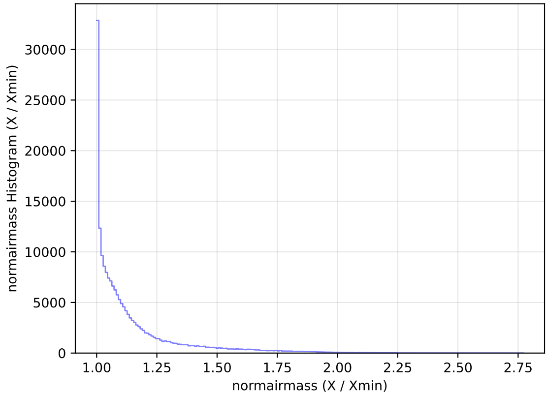
internal_u_expt45_nscale0.9v3.4_10yrs WFD g band: normairmass Histogram
