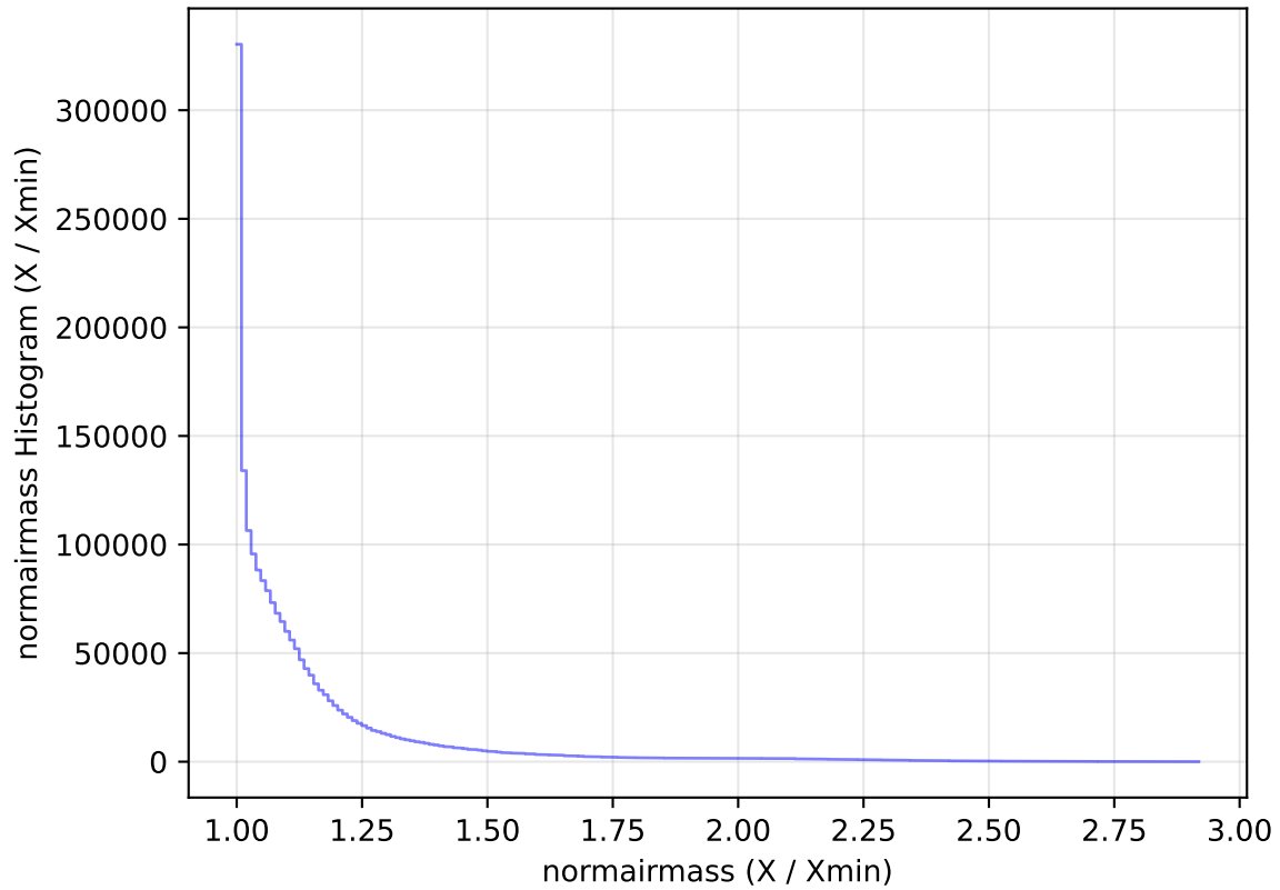
internal_u_expt45_nscale0.9v3.4_10yrs WFD all bands: normairmass Histogram
