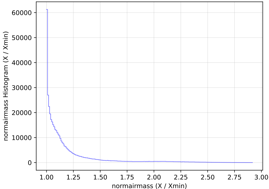
internal_u_expt45_nscale0.9v3.4_10yrs All sky z band: normairmass Histogram
